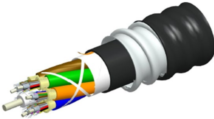
Indoor/Outdoor Plenum Aluminum Interlocking Armor Distribution Cable positioned for indoor and outdoor use.
