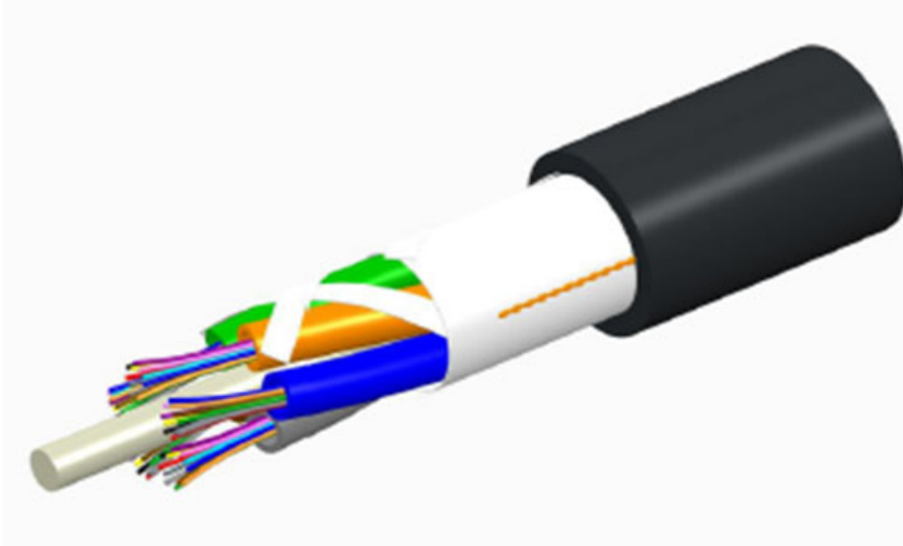
Indoor/Outdoor LSZH Single Jacket All-Dielectric Cable for indoor or outdoor use
