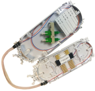
FOSC® 450 Fiber Optic splice tray kit with one 2-port Tray Tap, 5 dB
