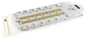
FOSC® D Splice Tray, 6 splice modules, 72-splice capacity
