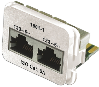
AMP CO Plus Insert, 2-port RJ45, category 6A ethernet, almond
