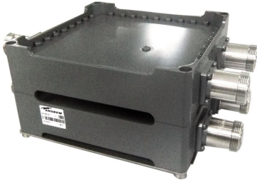
Twin Crossband Coupler, Cellular/900 MHz/DCS 1800/PCS/AWS
