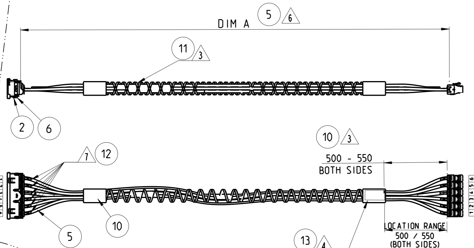
SCHEMATIC VIEW (FOR REFERENCE ONLY)
