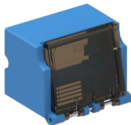
LC Duplex Low Profile Adapter Shutter Assembly, blue with collar with opaque shutter
