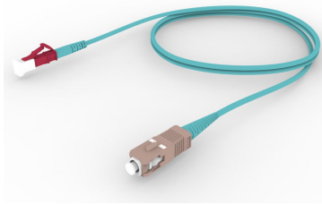
OM4 LC/UPC Keyed Red to SC/UPC Fiber Patch Cord, 1.6 mm Simplex, Riser
