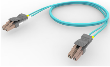
OM4 LC/UPC to LC/UPC Fiber Patch Cord, 1.6 mm Duplex, Plenum, Slate (AC) Locking Clip
