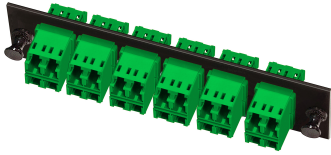
Fiber Optic Snap-in Adapter Pack, singlemode, LC, 24-fiber, green, loaded
