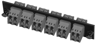
Fiber Optic Snap-in Adapter Pack, multimode, LC, 24-fiber, black, loaded
