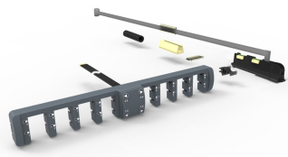
SYSTIMAX 360™ iPatch® 32-MPO UHD Shelf, 6PK imVision Upgrade Kit
