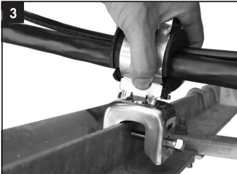
Insert SnapStak hanger into 3/4" mounting hole adapter or cable ladder. SnapStak hangers can be stacked 2 high maximum.
