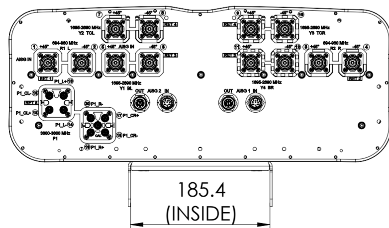
VIEW A-A SCALE 1 : 5
