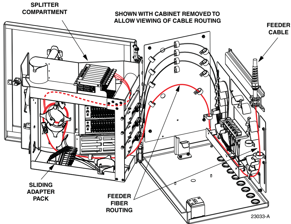
Figure 10. Factory-Installed Feeder Cable Configuration - Top Entry
