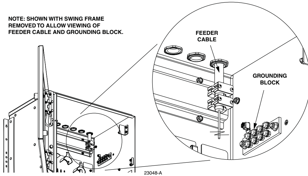
Figure 14. Location of Cable Grounding Block
