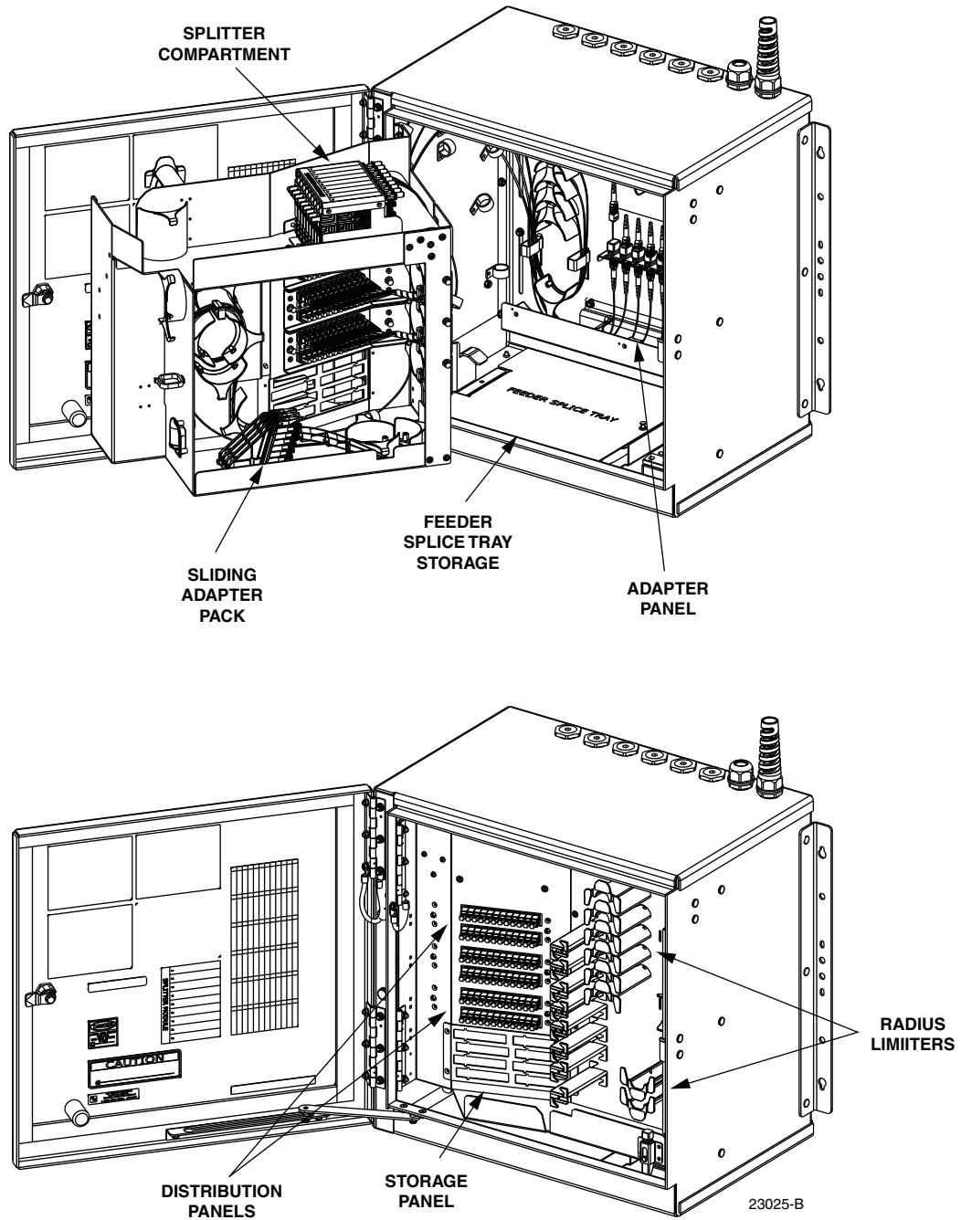
Figure 1. Typical FDH 3000 Indoor 72 Cabinet With Multi-Fiber Distribution Connectors
