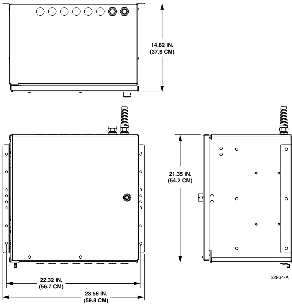
Figure 2. FDH 3000 Indoor 72 Cabinet With Multi-Fiber Connectors Dimensions
