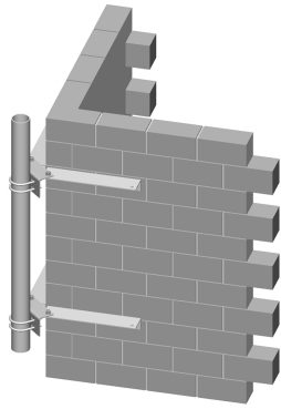
Corner Wall Mount, 2-3/8 in OD x 96 in pipe
