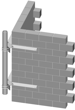
Corner Wall Mount, 2-3/8 in OD x 96 in pipe
