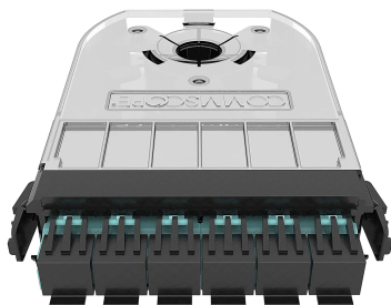
360G2 Cassette 12 LC Multimode OM4 Aqua iPatch Ready
