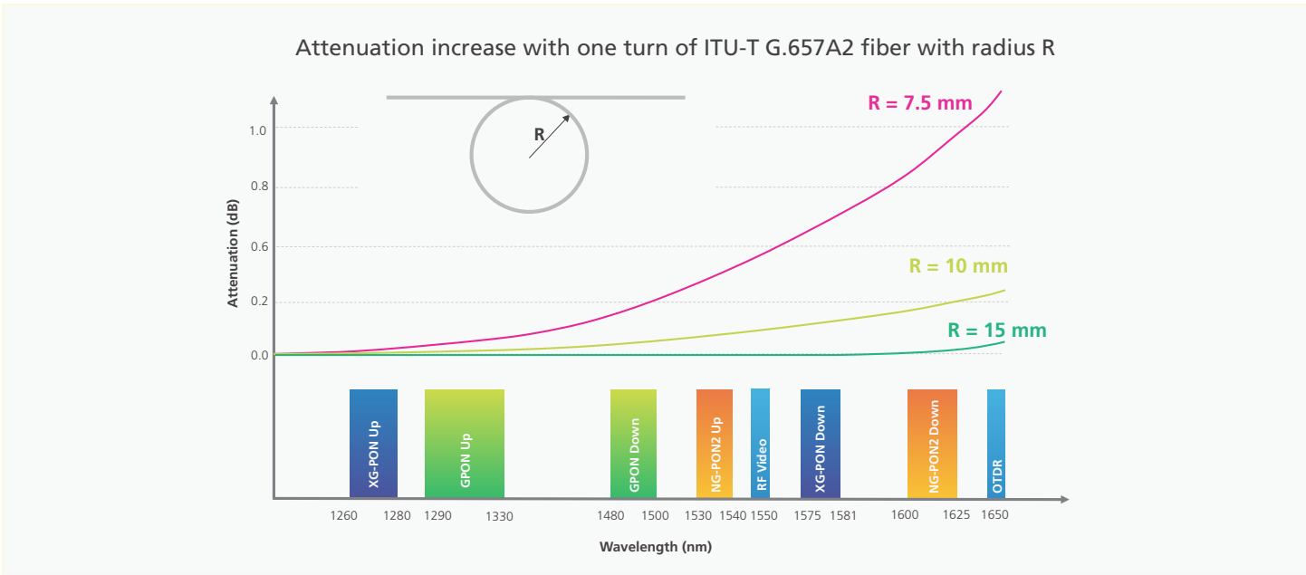
Figure 6: Macrobending attenuation for ITU-T G.657 A2 fiber
